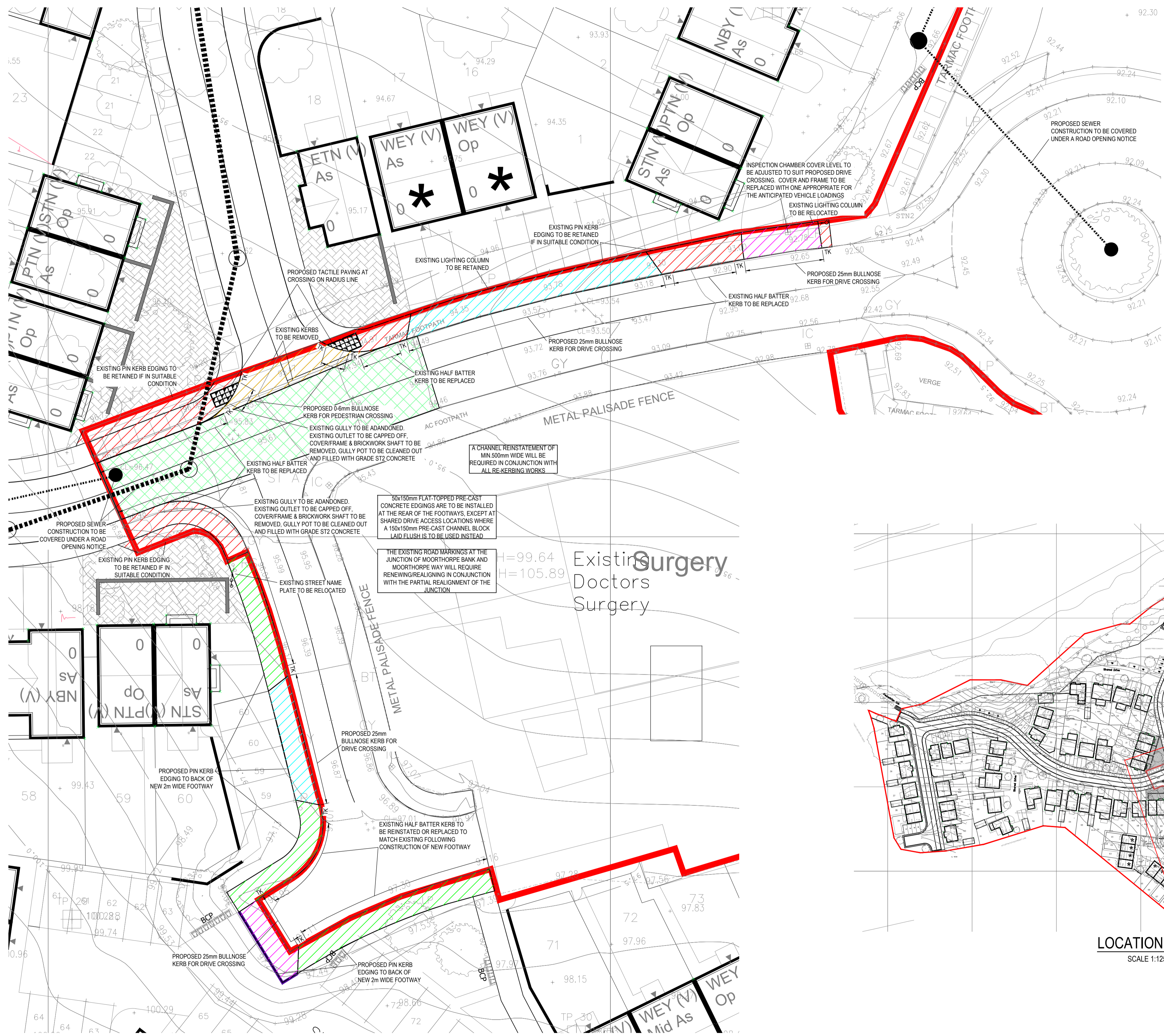
SECTION 278 WORKS SCALE 1:200
